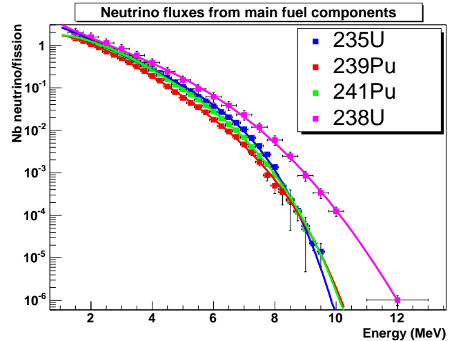
FIG. 7: Measured spectra of antineutrinos from the main components of the nuclear fuel. Taken from Ref. [20].
