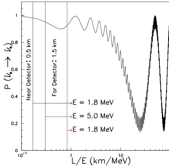
FIG. 3: Antineutrino survival probability P(\bar{\nu}_e \rightarrow \bar{\nu}_e) as function of the ratio L/E [km/MeV]. Vertical lines indicate some relevant reactor neutrino energies. E = 1.8 \text{ MeV} corresponds to the reaction threshold. The peak of the energy spectrum weighted by the detection cross section in the absence of oscillation is at E \sim 4 \text{ MeV} , and the contribution of neutrinos with energy \lesssim 5 \text{ MeV} is the most important.
