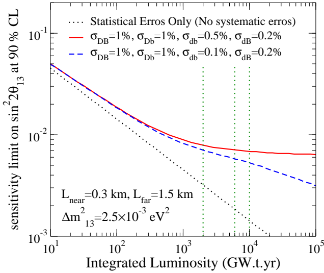
FIG. 5: Sensitivity limit as a function of the integrated luminosity. Vertical dashed lines represent 1, 3 and 5 years of data taking.
