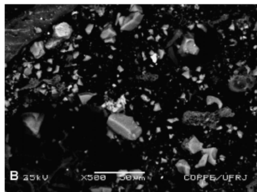
Fig. 2. General view of manually ignited 9 mm Luger primer from CleanRange® first (A) and second (B) generation ammunition collected onto double-face carbon tape pin mounts.
